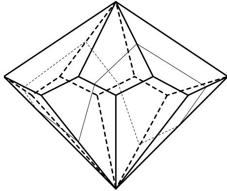
FIG. 4.1. Flying saucer (of degree 2) and a canonical surface in it.
