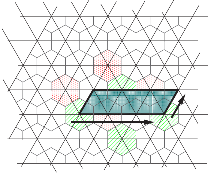
FIG. 3.2. Coloured horosphere tessellation.
