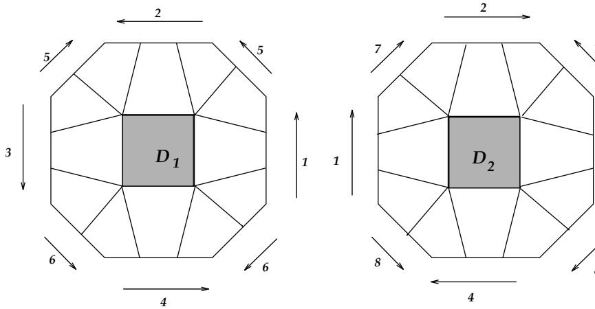
FIG. 2.1. Squared Genus-2 Surface.
