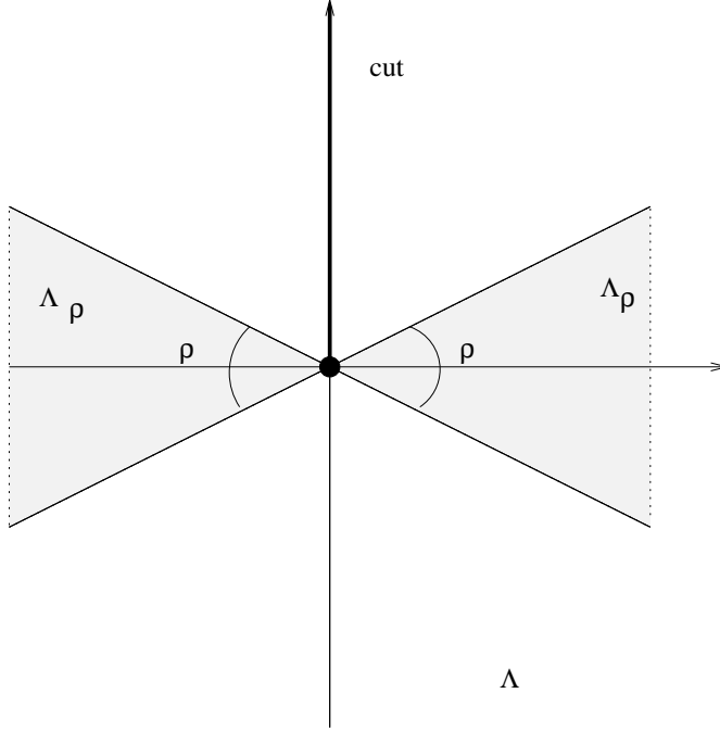
FIG. 1. Conic neighbourhoods of the real axis on the logarithmic plane.
