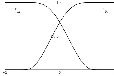
FIGURE 2: CUTOFF FUNCTIONS
