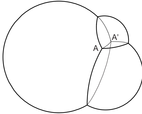
FIG. 3. Standard 3-bubble in \mathbb{R}^2 blown to \mathbb{R}^3
