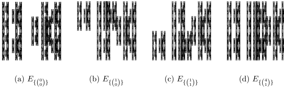
FIG. 2. c -vector \mathcal{E} = A(M)
