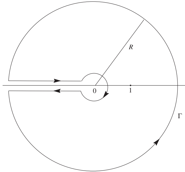
FIGURE 1. Contour \Gamma
