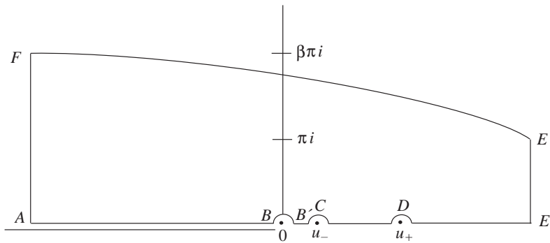
FIGURE 5. u -plane ( \beta > 1 )
