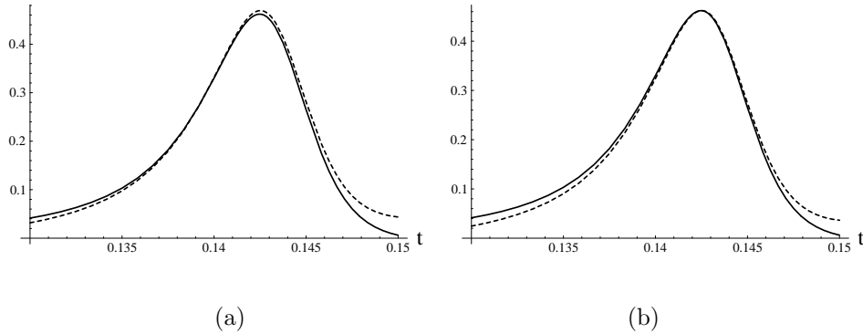
FIGURE 5.1. In both figures, the solid curve is the graph of the left side of (5.2) using t_0 = .14 and \alpha = .0011339931265054 computed using (5.1); see Table 1. The dashed curves depict the right side of (5.2), with (a) having B = x_j = -.151 and (b) having B = B_b = -.1689 . For larger values of t_0 , the agreement is even better.
