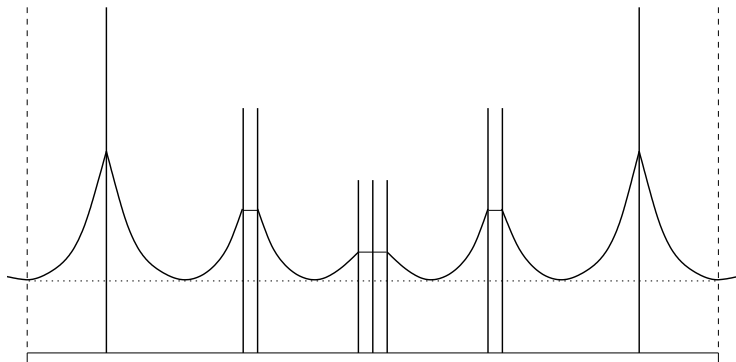
FIG. 1.2. A schematic illustration of a finite part of the pattern (U_{A_1A_2A_3A_2A_1}^{\text{per}}(x), V_{A_1A_2A_3A_2A_1}^{\text{per}}(x)) associated to an A_1A_2A_3A_2A_1 -orbit of \tau\sigma\tau^{-1} -type (with \tau = A_1A_2 , \sigma = A_3 ). The 'full' pattern can again be obtained by reflection with respect to the boundaries of the domain. The singular V -pulses are represented by vertical line segments. The U -components are, to leading order, constant during the fast excursions of \gamma_{A_1A_2A_3A_2A_1}^{\text{per}}(\xi) . Note that the values of U are identical at the minima of U_{A_1A_2A_3A_2A_1}^{\text{per}}(x) (up to exponentially small corrections, see section 3).
