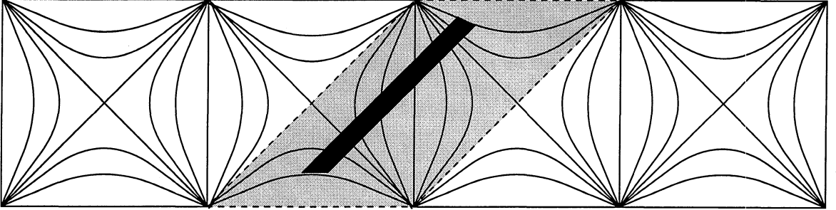
Figure 1: The lightly shaded region indicates the universal cover of an open 1+1 de Sitter annulus with hyperbolic holonomy which is not a domain of dependence. The darker region is a fundamental domain for compact annulus with spacelike boundary.
