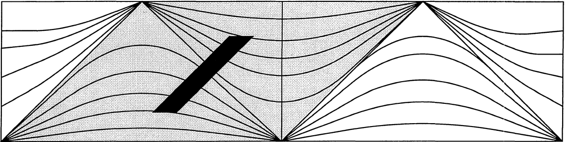
Figure 2: The lightly shaded region indicates the universal cover of an open 1+1 de Sitter annulus with parabolic holonomy which is not a domain of dependence. The darker region is a fundamental domain for compact annulus with spacelike boundary and no closed timelike curves.
