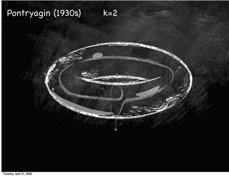
FIGURE 4. The nonlinearity of \varphi . Even if the framing on the torus is such that its restrictions to the longitudinal and latitudinal circles each extends to a disk, the resulting framing on their sum does not.
