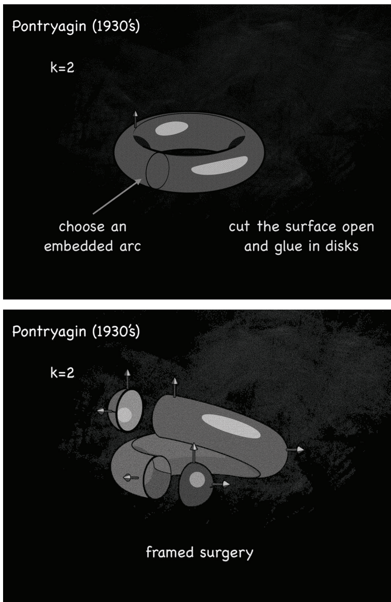
FIGURE 3. The case k = 2 and genus 1. If the framing on the embedded arc extends to a disk, then there is a cobordism (called a framed surgery) that converts the torus to a 2-sphere as shown.
