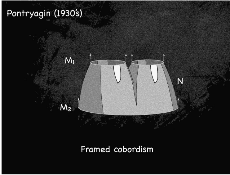
FIGURE 1. A framed cobordism between M_1 = S^1 \amalg S^1 \subset \mathbf{R}^2 and M_2 = S^1 \subset \mathbf{R}^3 with N \subset [0, 1] \times \mathbf{R}^2 . The normal framings on the circles can be chosen so they extend over N .
