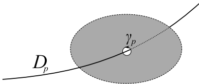
FIGURE 4. Holomorphic maps (in grey) with an asymptotic condition along the orbit \gamma_p linking D_p , correspond to holomorphic maps with an intersection point with D_p
