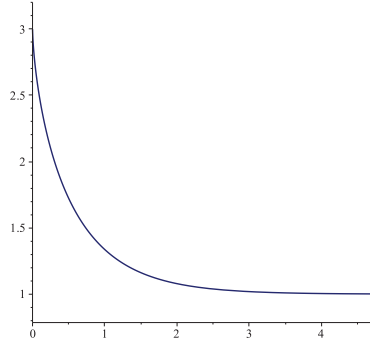
FIGURE 2. Plot of the function \phi(x) for m = 1 , s = 3 , and M = 5 .
