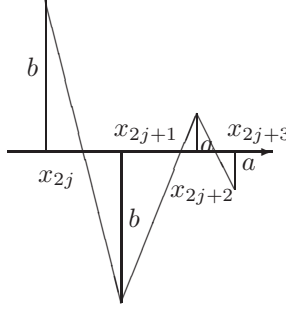
FIGURE 1. An illustration of the piecewise linear function u
