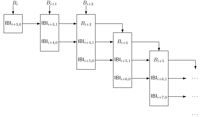
Figure 2. Illustration of quantities which can be computed simultaneously for k=3 .
