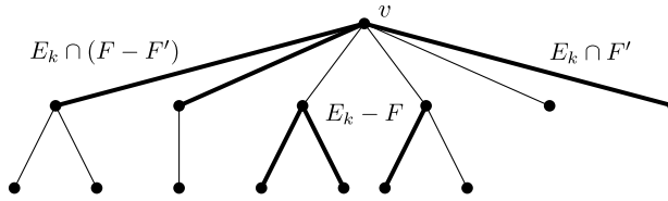
Figure 1: The set E_k for Proposition 3.1.
