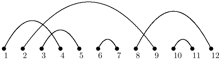
Figure 1: The diagram of the matching M = \{(1, 4), (2, 9), (3, 5), (6, 7), (8, 12), (10, 11)\} .
