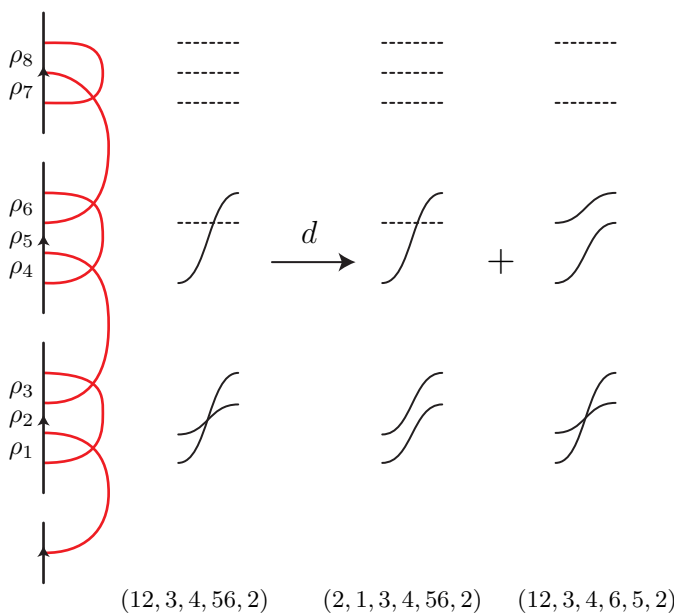
Figure 5. The differential of the algebra element (12, 3, 4, 56, 2) .
