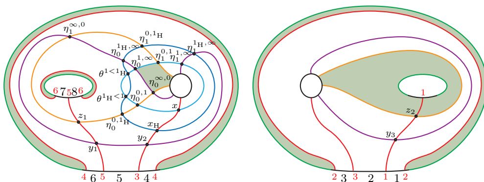
Figure 9. The bordered-sutured multi-diagram
