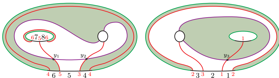
(B) The bordered-sutured diagram \mathcal{H}_\infty .
