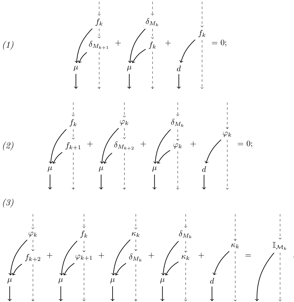
Figure 2. Graphical representations of the conditions in Lemma 2.1.
