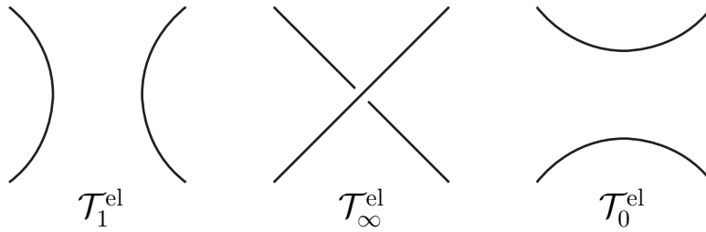
Figure 1. The elementary tangle \mathcal{T}_\infty^{\text{el}} and its resolutions \mathcal{T}_0^{\text{el}} and \mathcal{T}_1^{\text{el}} .
