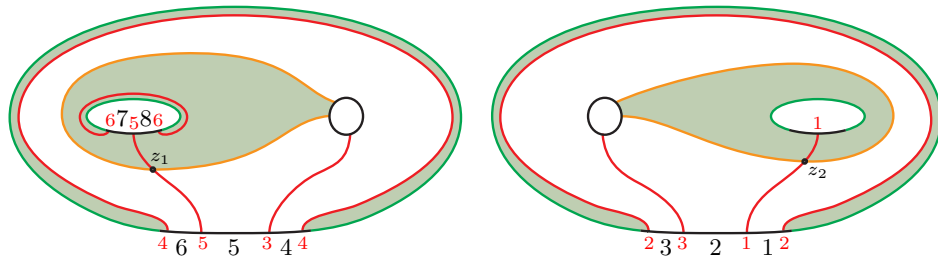
(C) The bordered-sutured diagram \mathcal{H}_0 .
