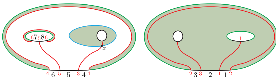
(A) The bordered-sutured diagram \mathcal{H}_1 .
