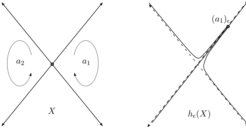
Figure 1: Action of h_\epsilon in a neighborhood of the base point for n = 2 .
